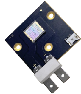
GT-FC300V405FC300A-4646B
